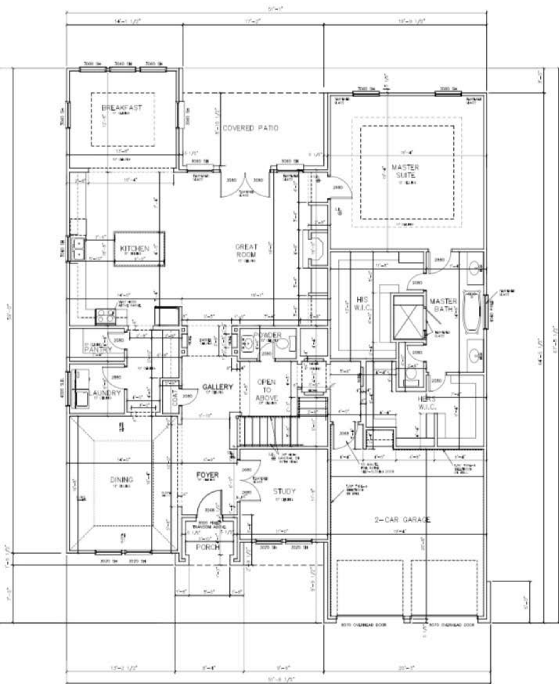
1st FLOOR LAYOUT
